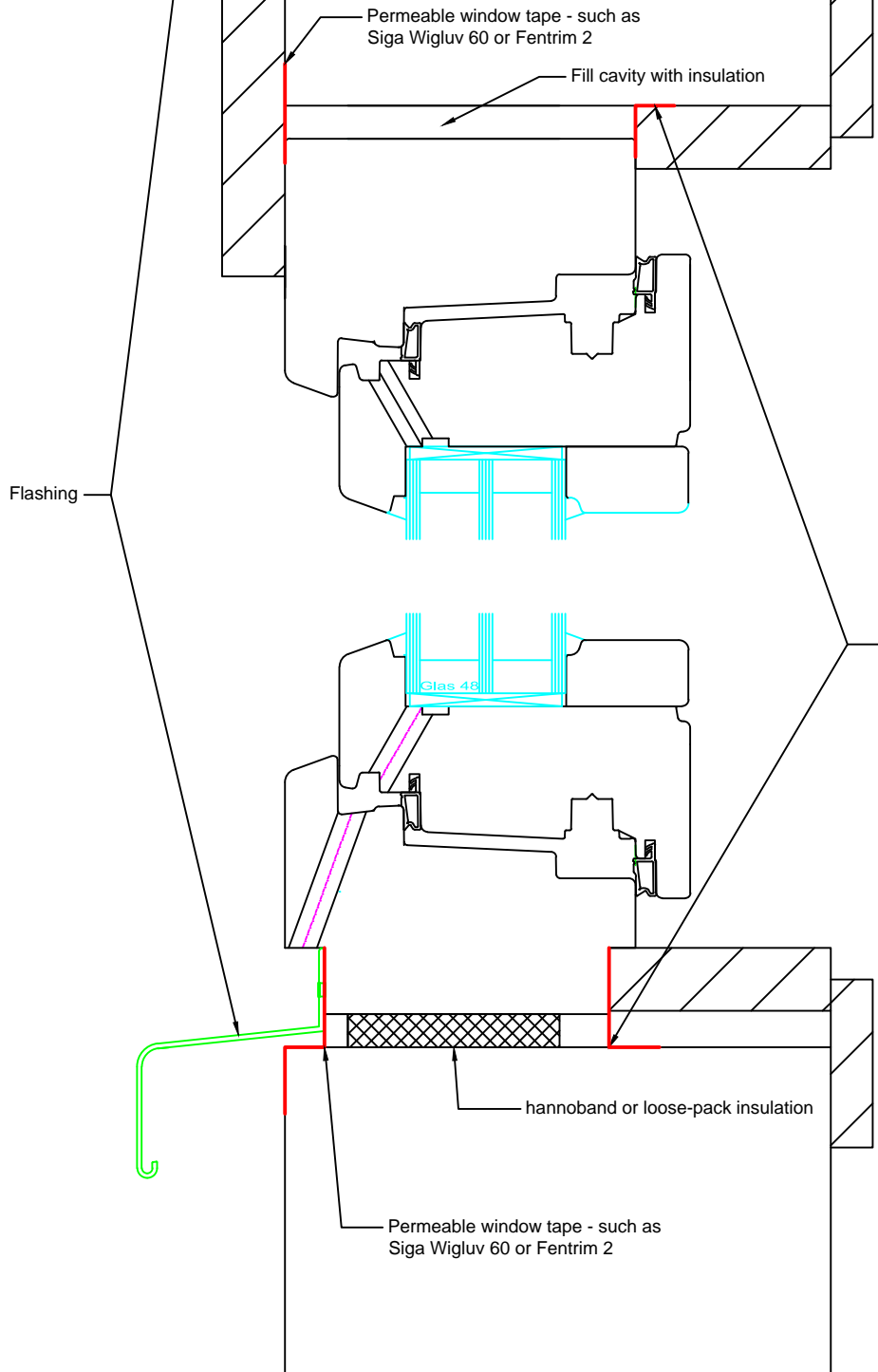
Installation Example - Flush with outside wall
